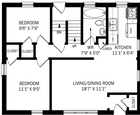
MAIN FLOOR - 740 SQUARE FEET
