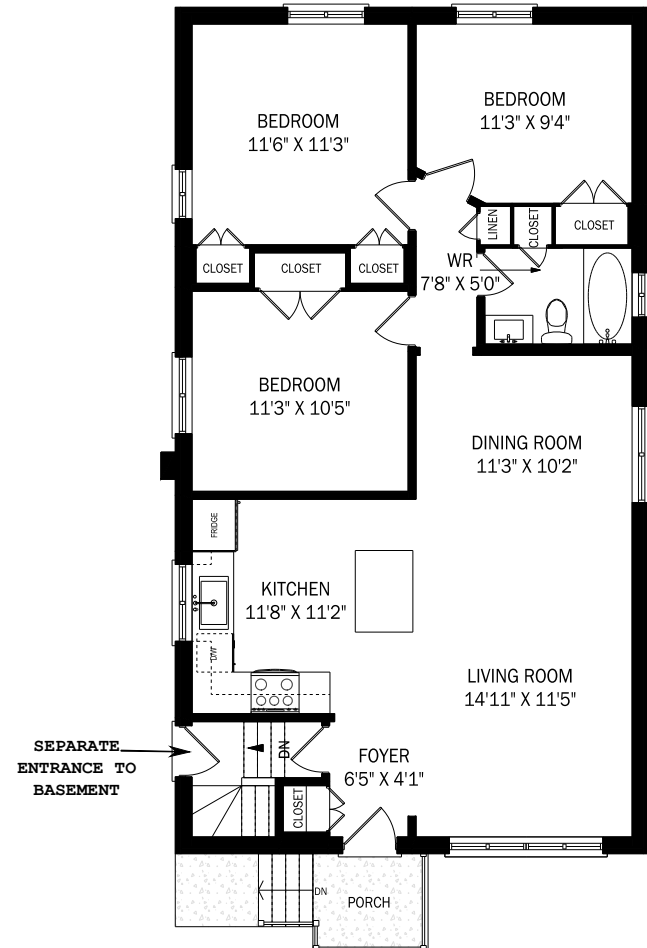
CEILING HEIGHT 8'0" MAIN FLOOR - 1087 SQUARE FEET
