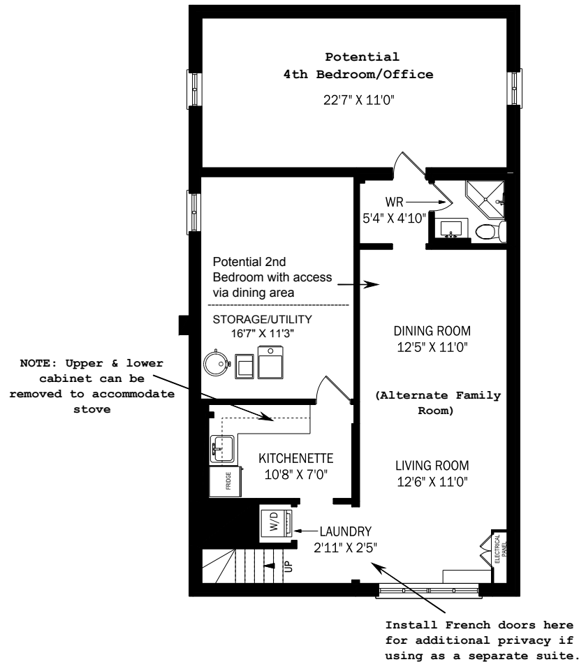
LOWER LEVEL - 1087 SQUARE FEET
