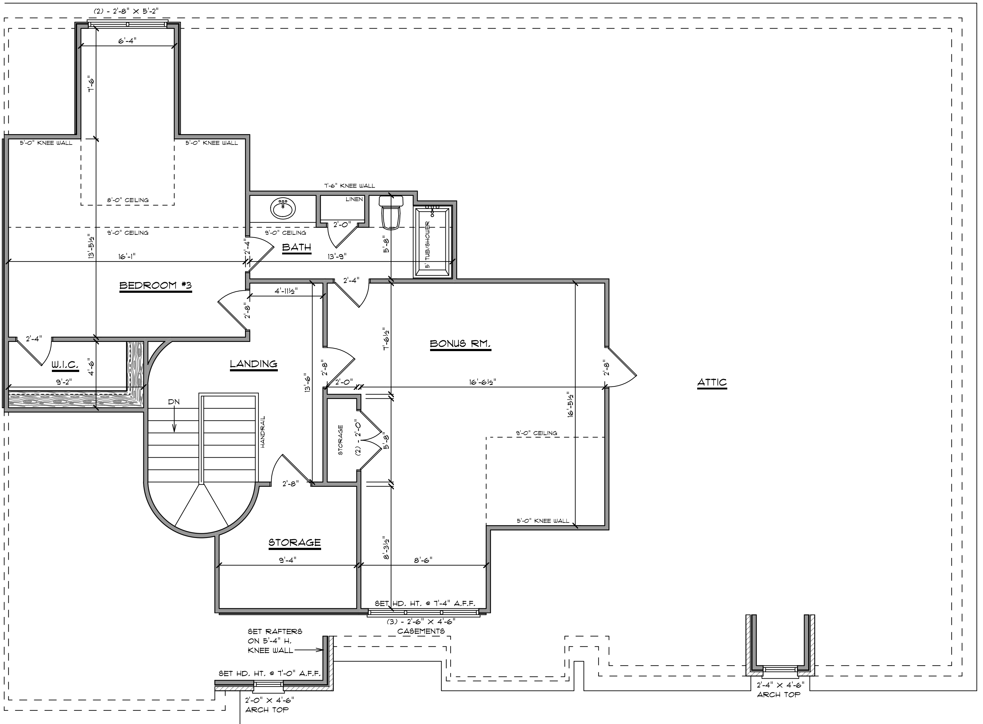
PROPOSED SECOND FLOOR PLAN SCALE: 1/4" = 1'-0"
