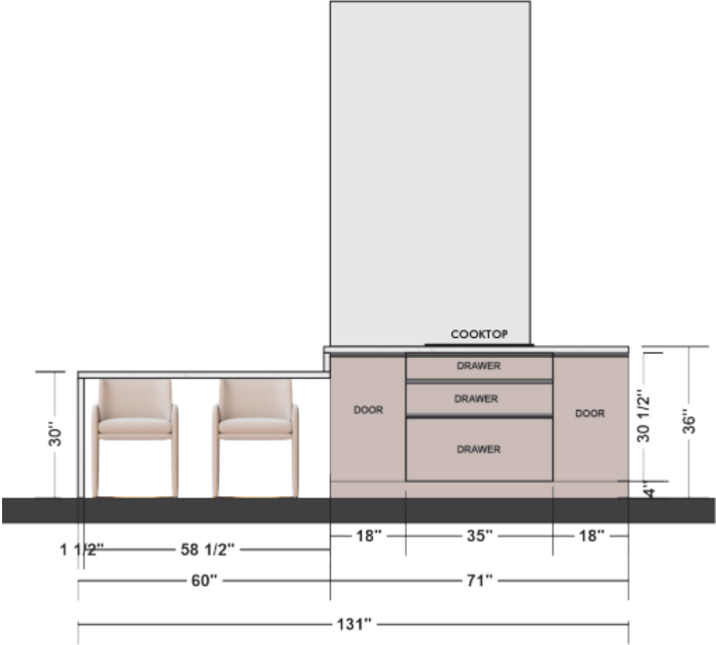
Elevation C
