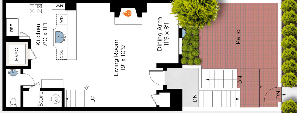
MAIN LEVEL 616 FIN. SQ.FT. 17 UNFIN. SQ.FT. 8'6" CEILING
