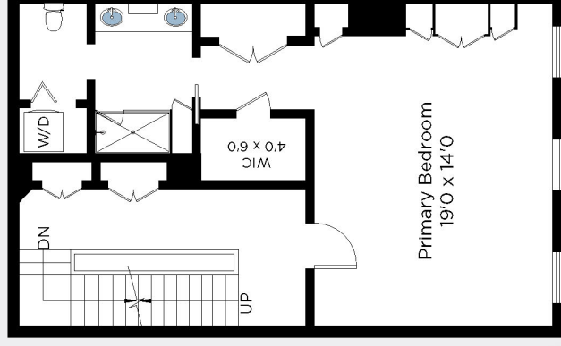
UPPER LEVEL 1 650 FIN. SQ.FT. 8' CEILING
