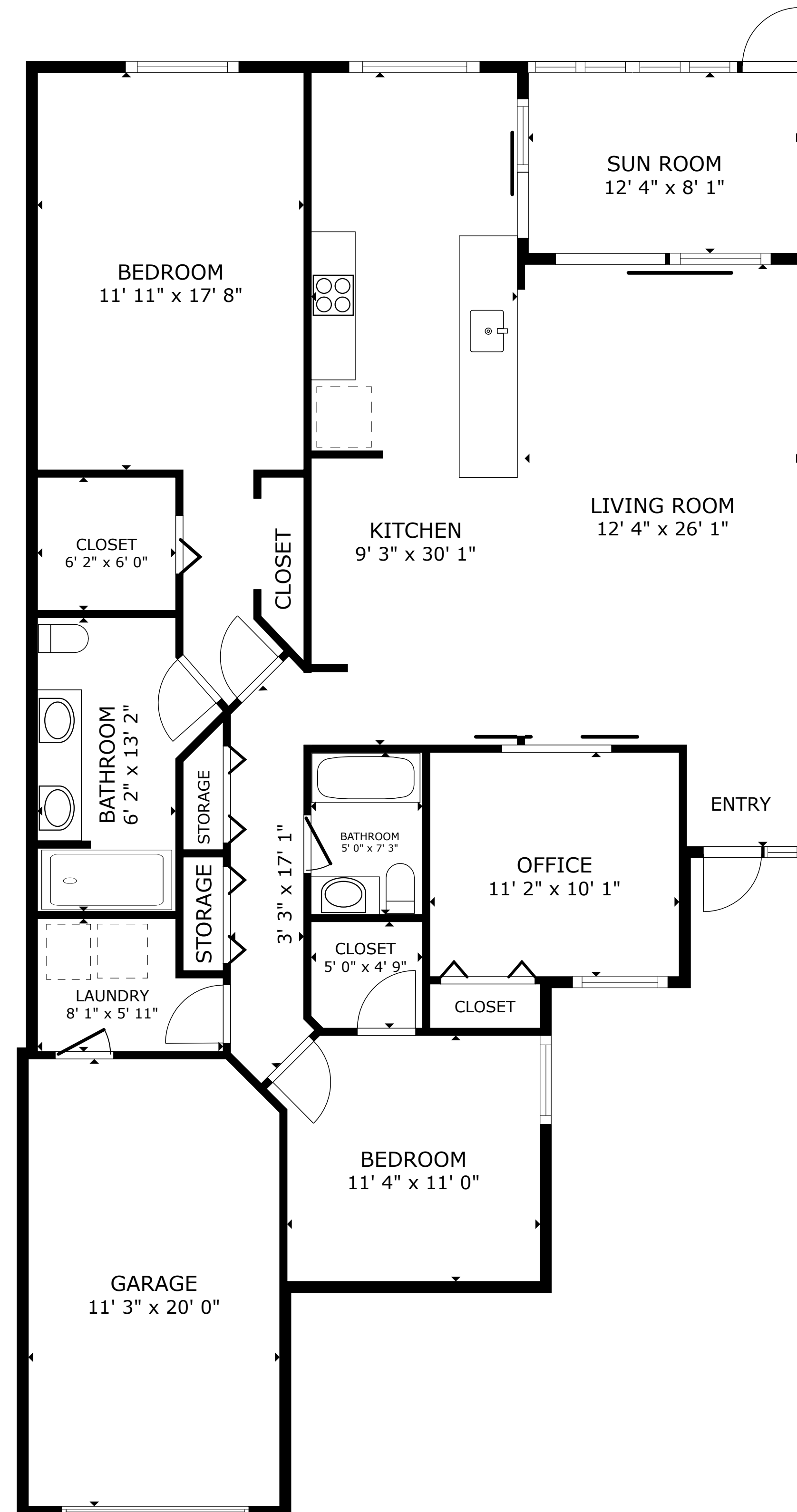
FLOOR PLAN
