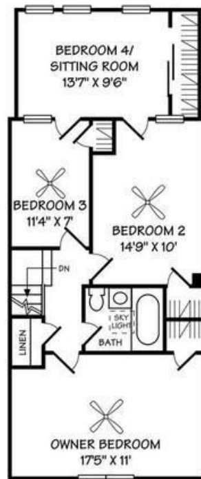
SECOND LEVEL
