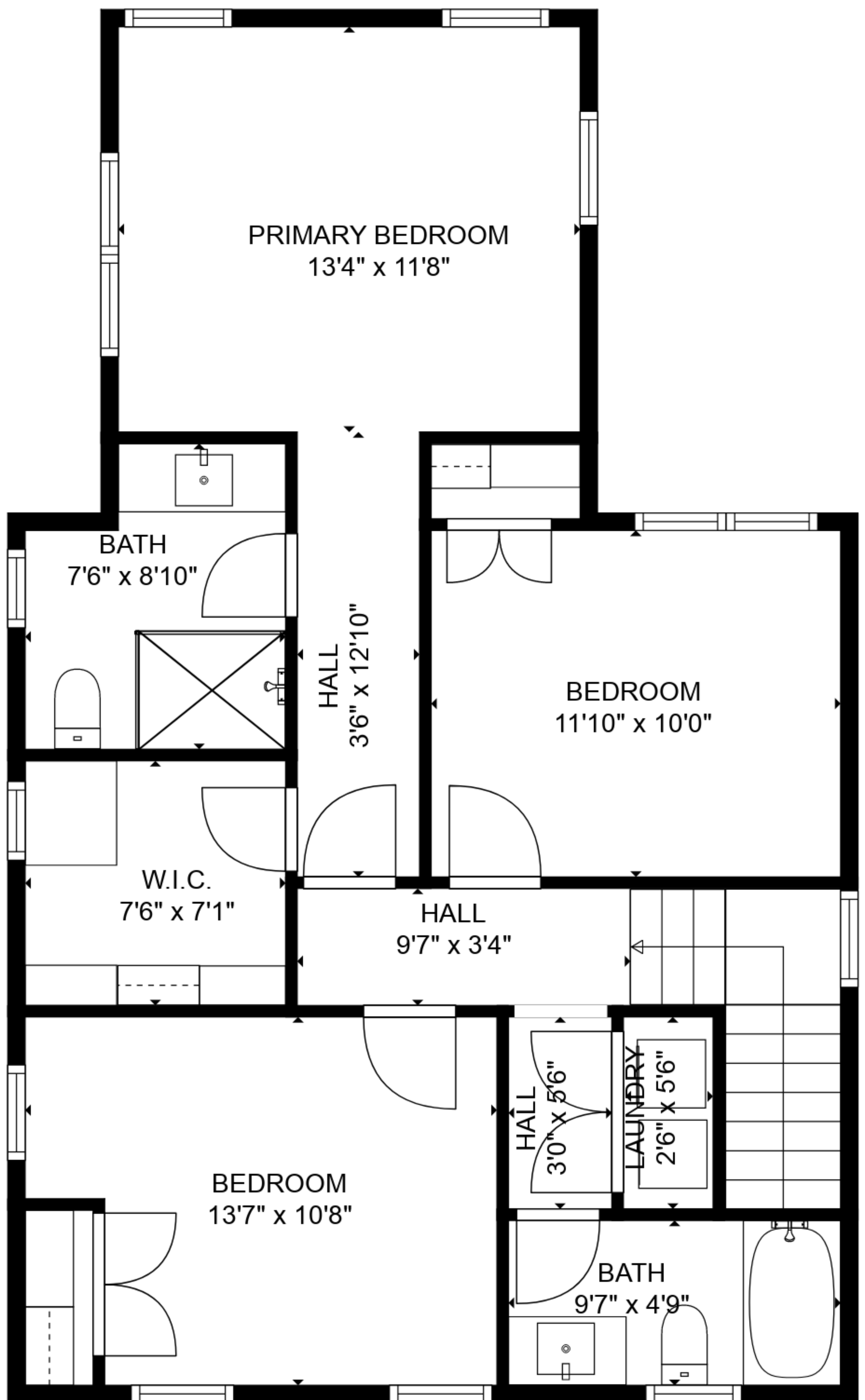
FLOOR 3
