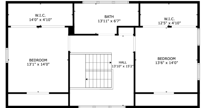
3rd floor
