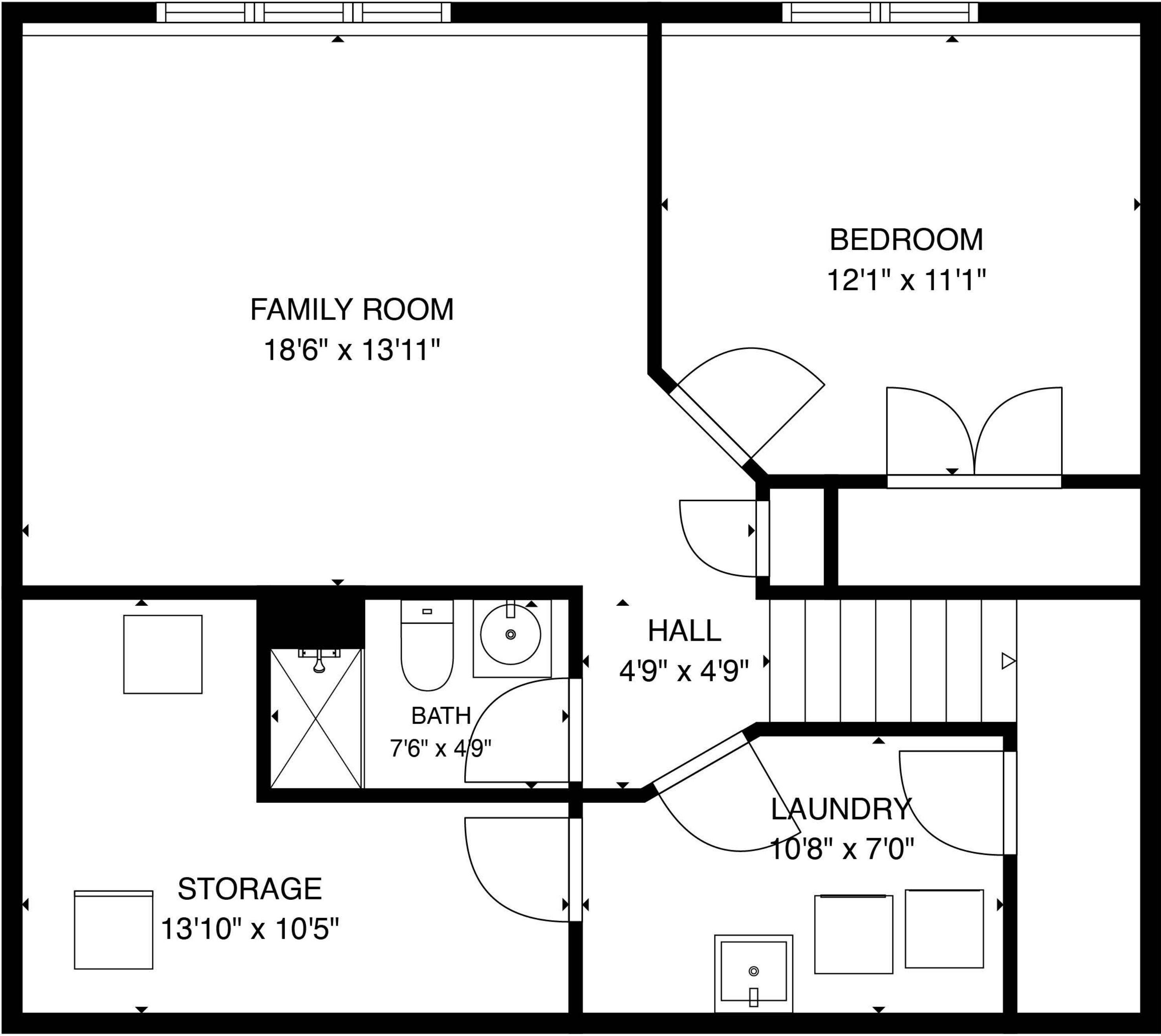
1st floor
