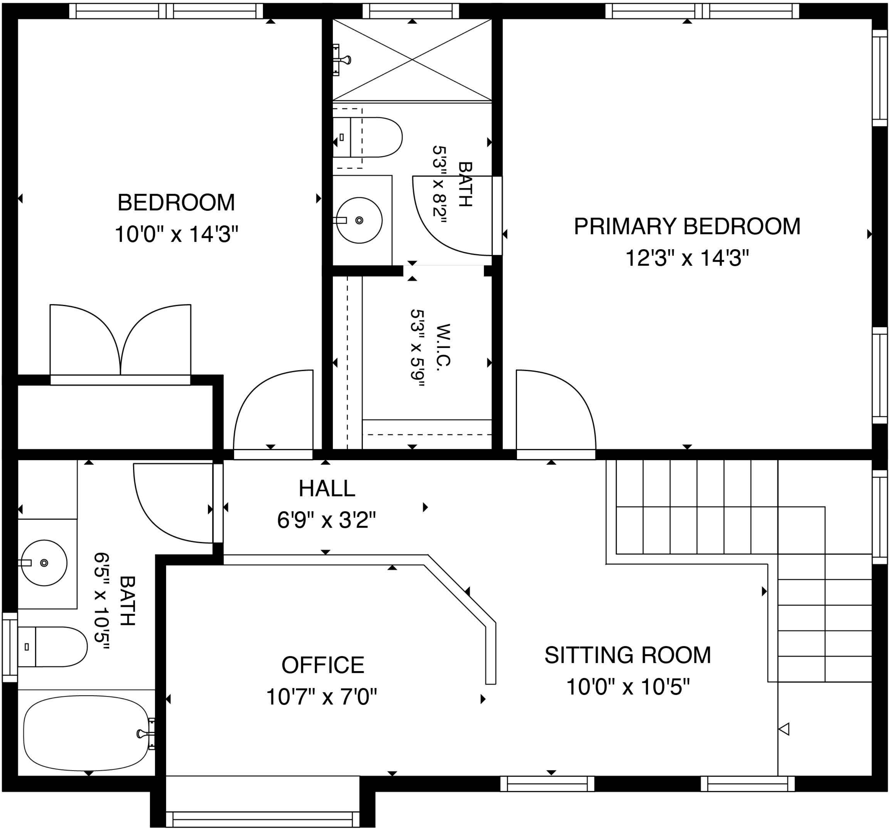
2nd floor
