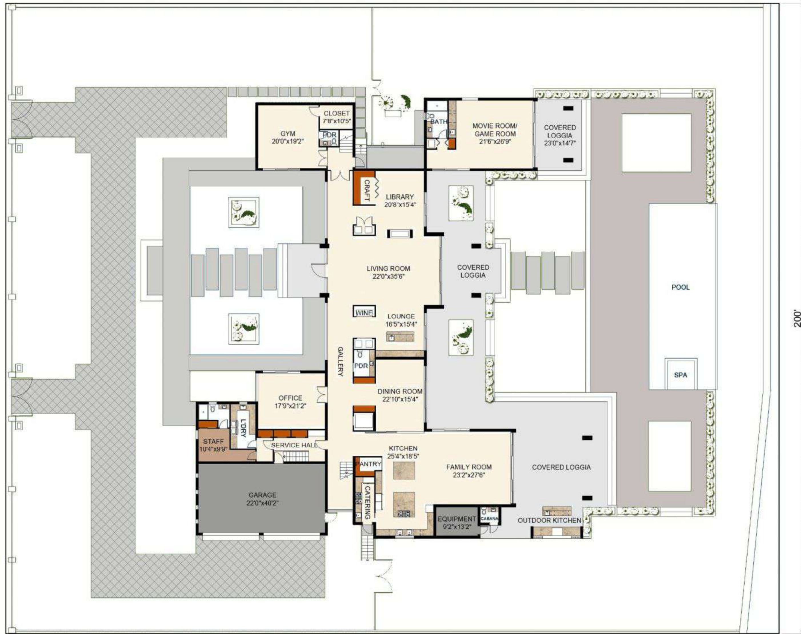
FIRST FLOOR SITE PLAN
