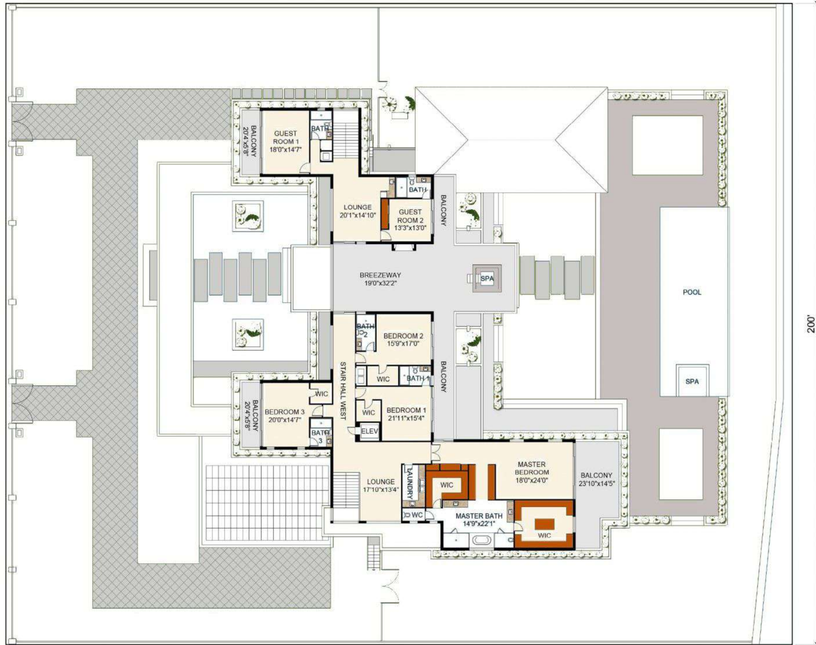
SECOND FLOOR SITE PLAN
