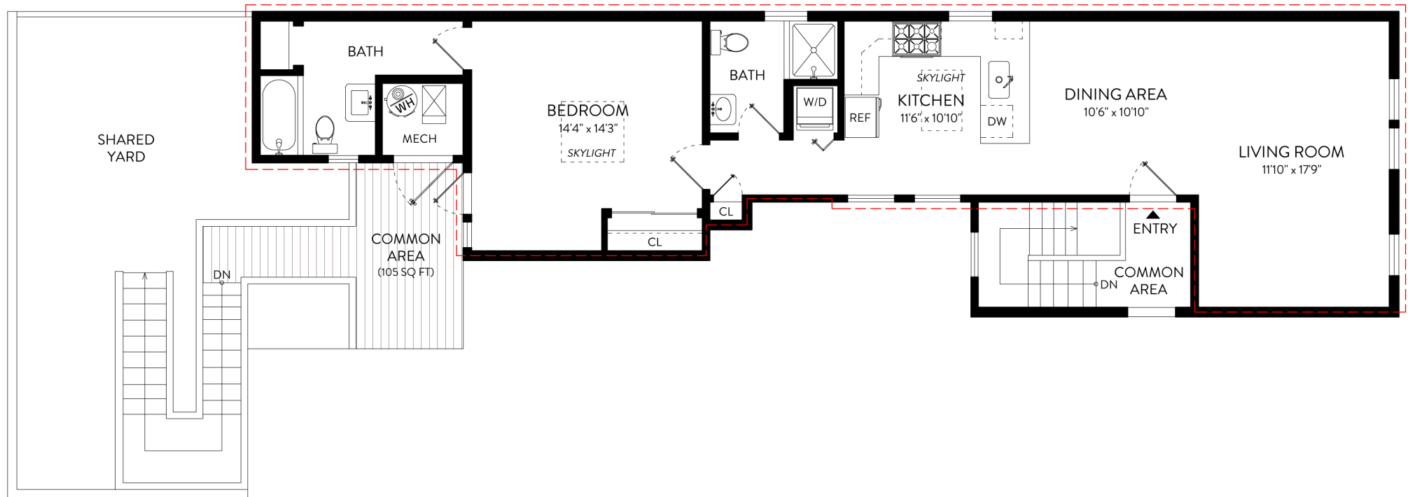
FLOOR PLAN
