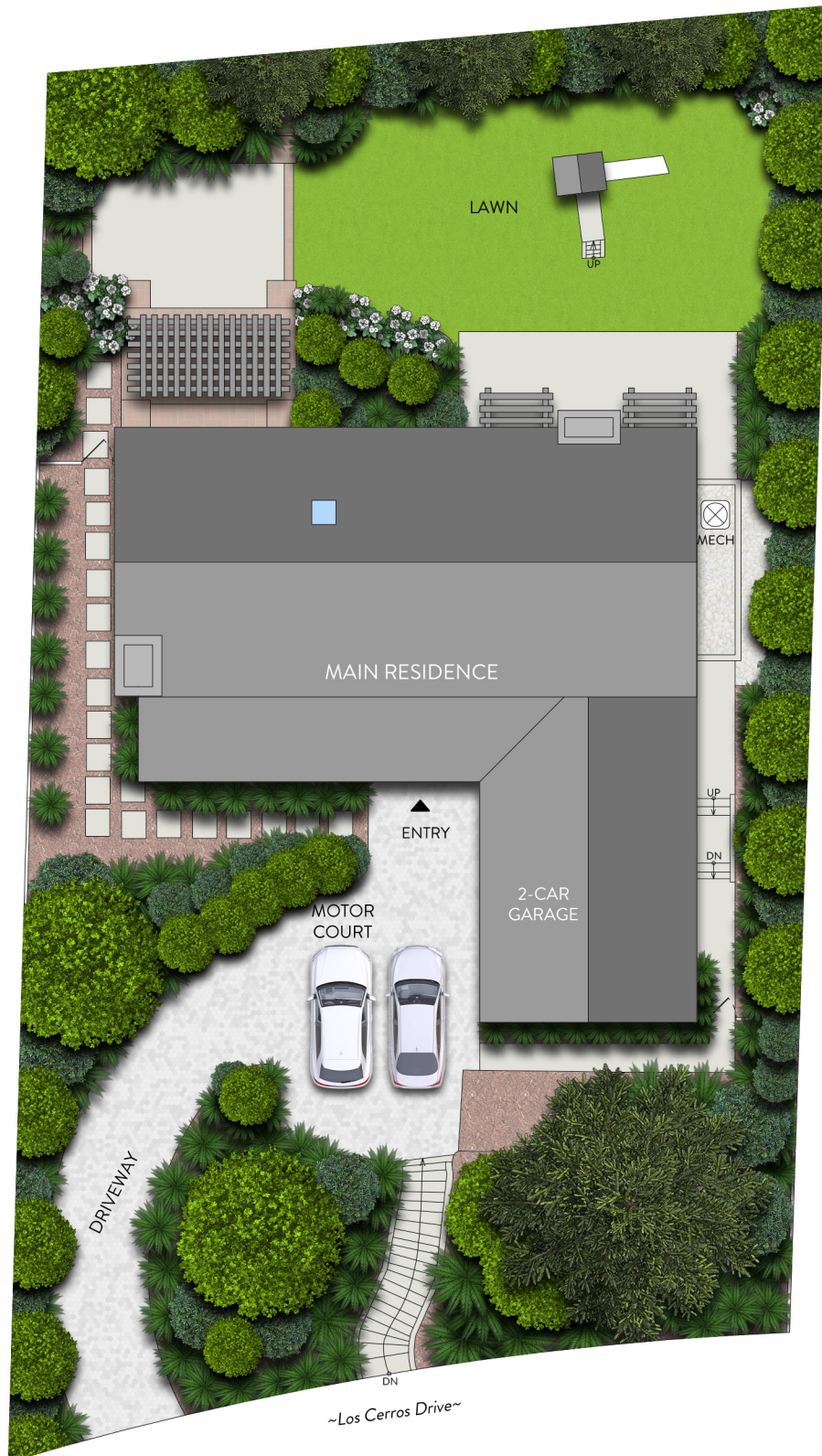
SITE PLAN
