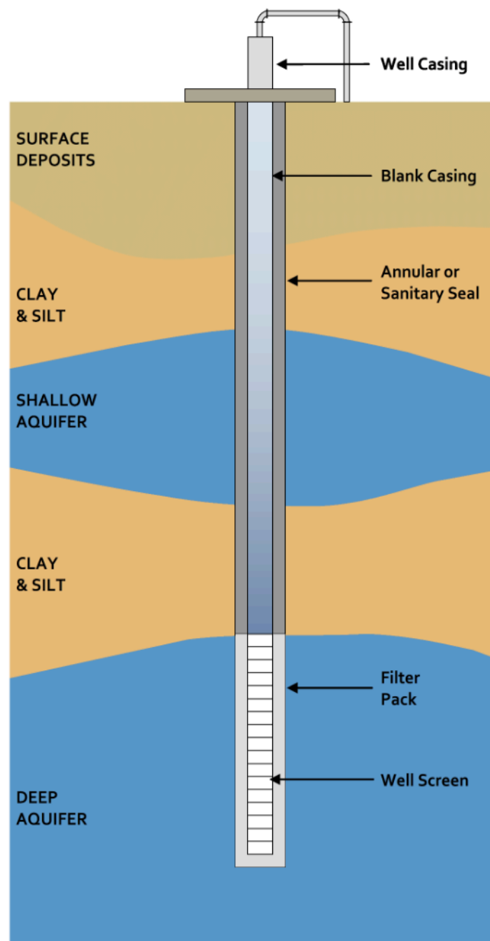
Figure 3: Typical well construction.
