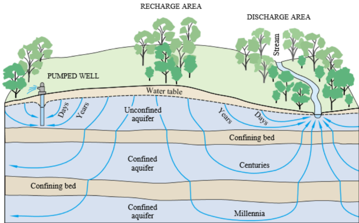
Figure 1: A typical, though simplified, groundwater system showing the different aquifer types and confining layers. Also shown are the average times for recharge to occur in the different aquifers.
