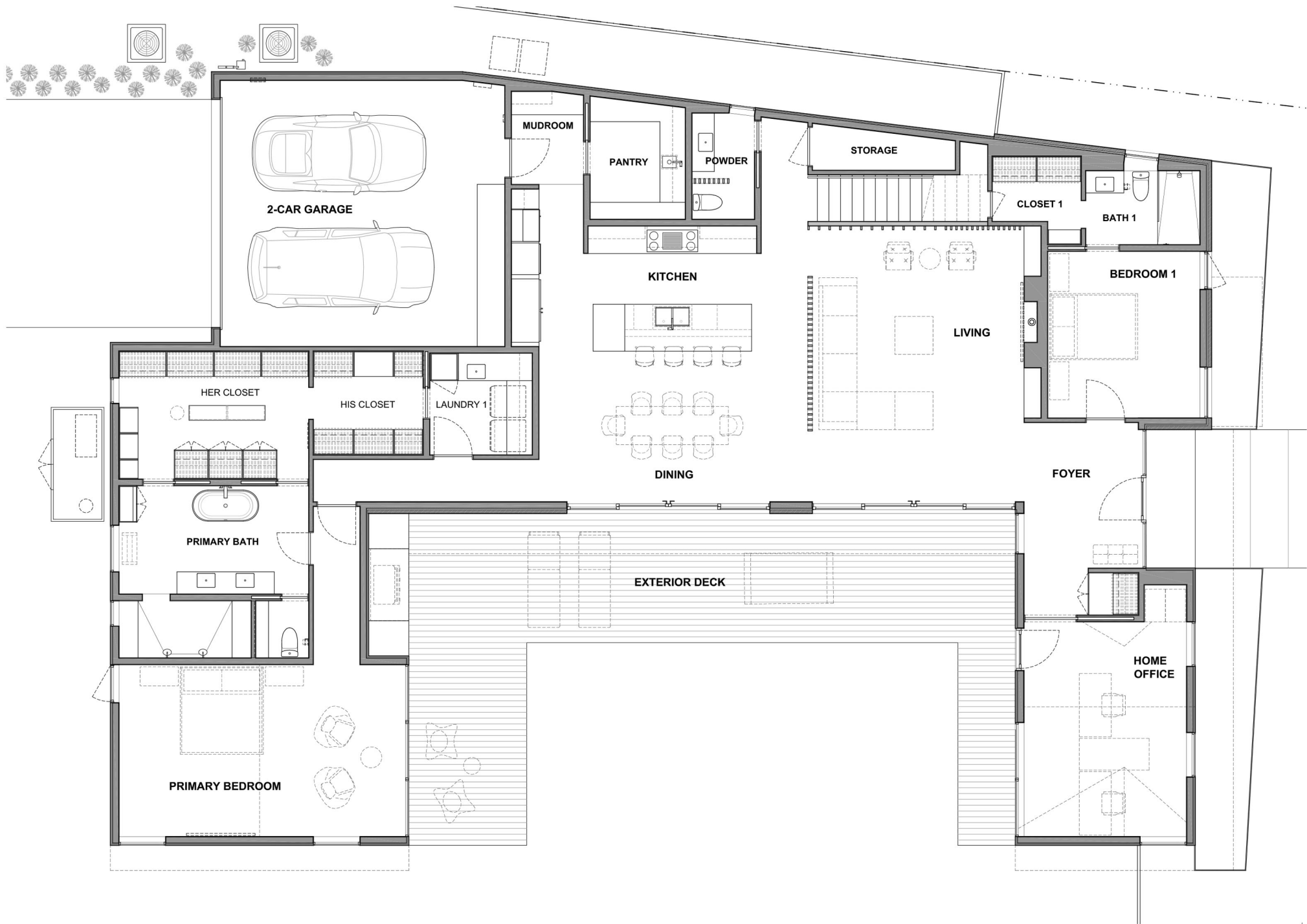
FLOOR PLAN / LEVEL 1
