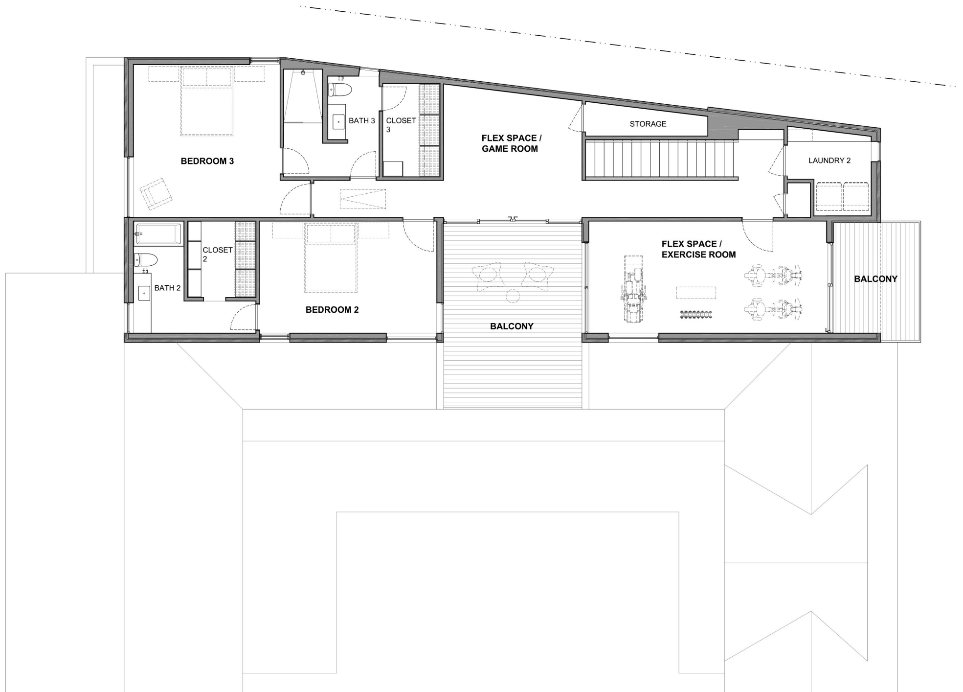
FLOOR PLAN / LEVEL 2
