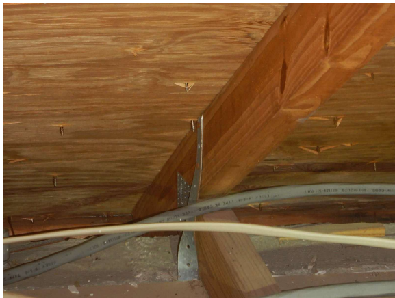
Roof to Wall Attachments – Straps
