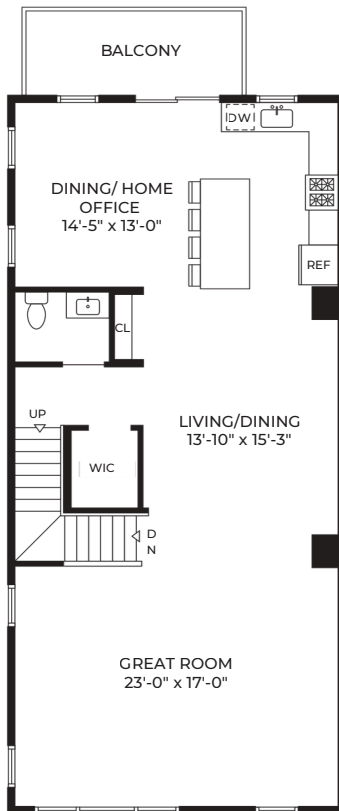
Second Floor
