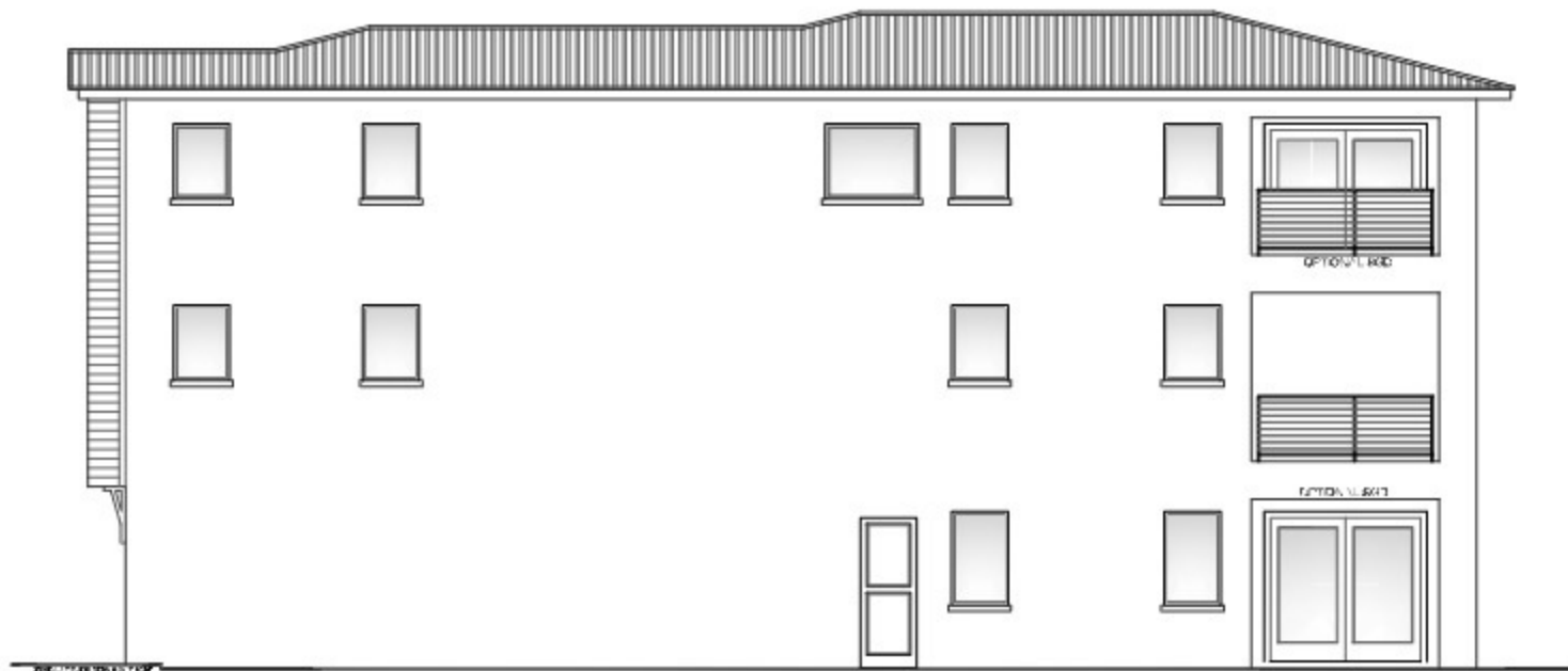
RIGHT ELEVATION THE SEACREST
