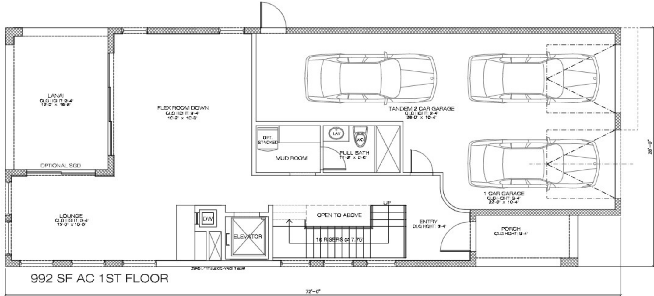
FIRST FLOOR PLAN THE SEACREST
