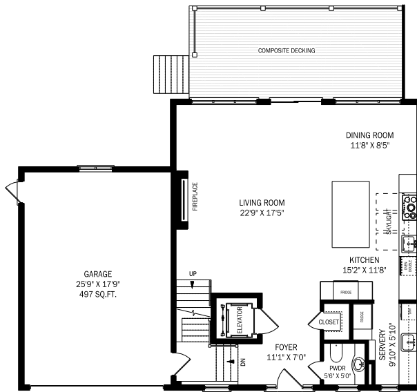
MAIN FLOOR - 1067 SQUARE FEET
