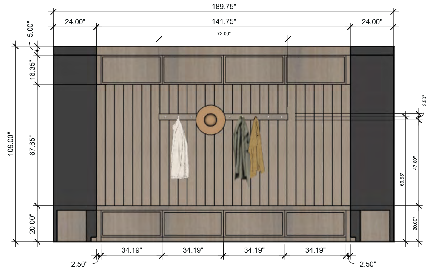
Mud Room Elevation 1 SCALE: 3/8" = 1'-0" (1:32)
