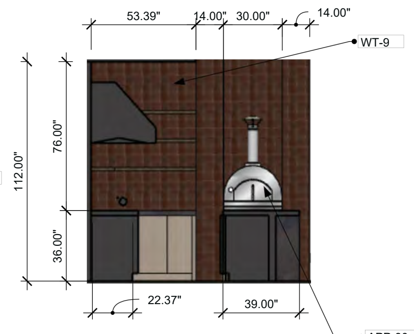
Outdoor Kitchen Elevation 2 SCALE: 1/4" = 1'-0" (1:48)
