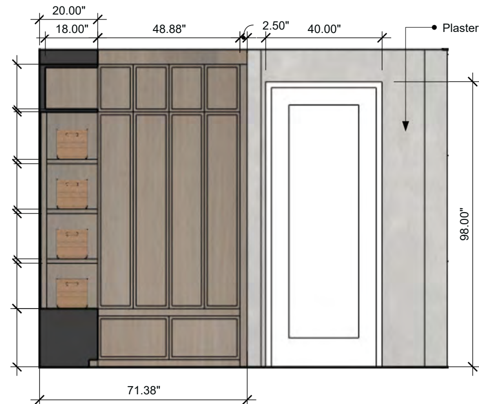
Mud Room Elevation 2 SCALE: 3/8" = 1'-0" (1:32)
