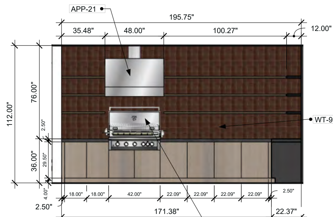
Outdoor Kitchen Elevation 1 SCALE: 1/4" = 1'-0" (1:48)
