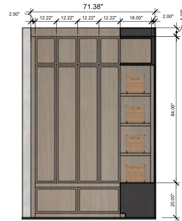
Mud Room Elevation 3 SCALE: 3/8" = 1'-0" (1:32)
