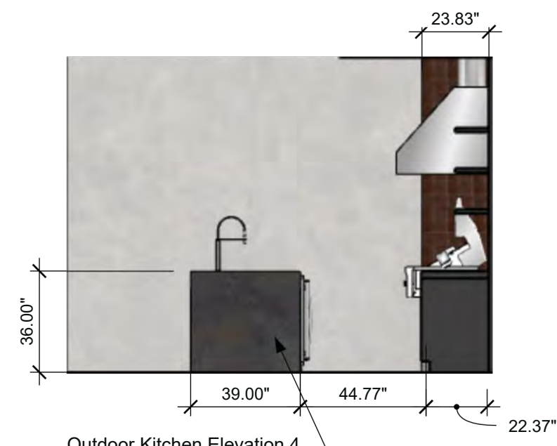
Outdoor Kitchen Elevation 4 SCALE: 1/4" = 1'-0" (1:48)
