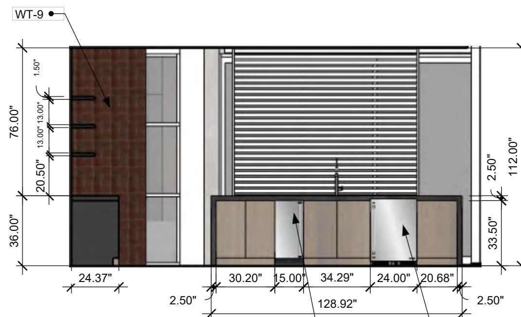
Outdoor Kitchen Elevation 3 SCALE: 1/4" = 1'-0" (1:48)
