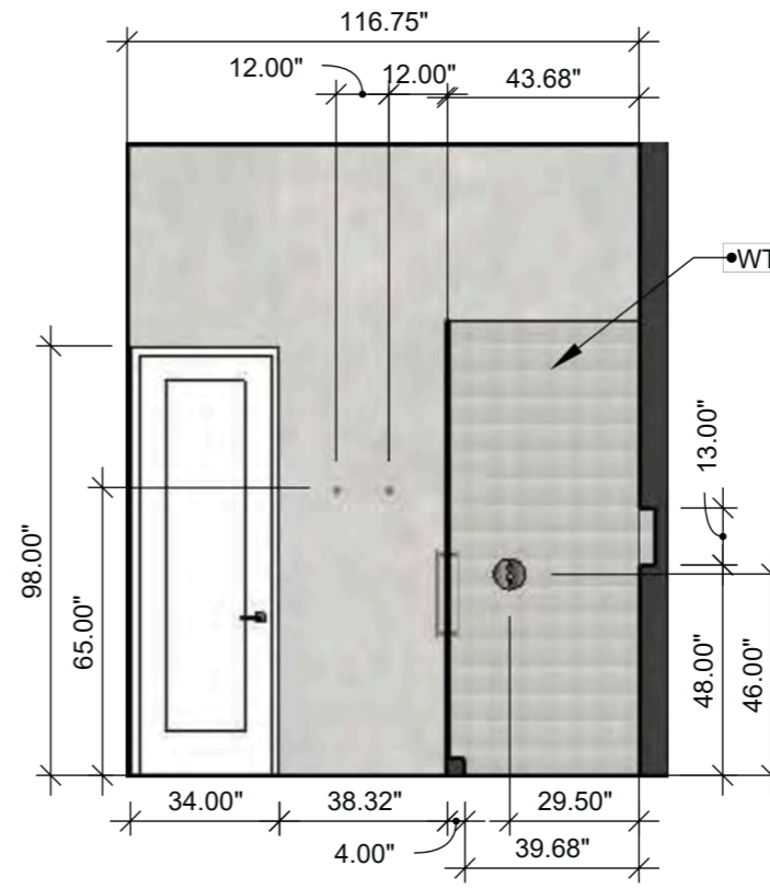
Outdoor Bath Elevation 3 SCALE: 1/4" = 1'-0" (1:48)
