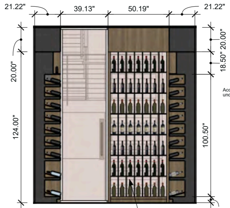
Wine Room Elevation 3 SCALE: 1/4" = 1'-0" (1:48)
