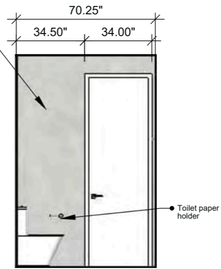
Shared Bath 1 & 2 Elevation 2 SCALE: 1/4" = 1'-0" (1:48)
