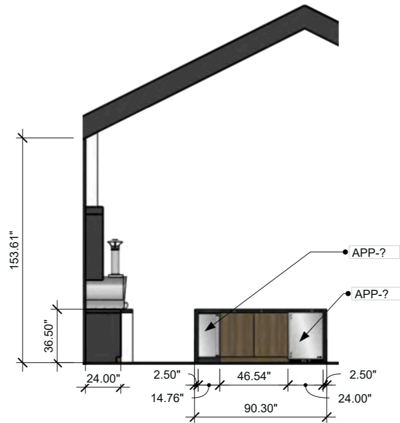
Outdoor Kitchen Elevation 3 SCALE: 3/16" = 1'-0" (1:64)
