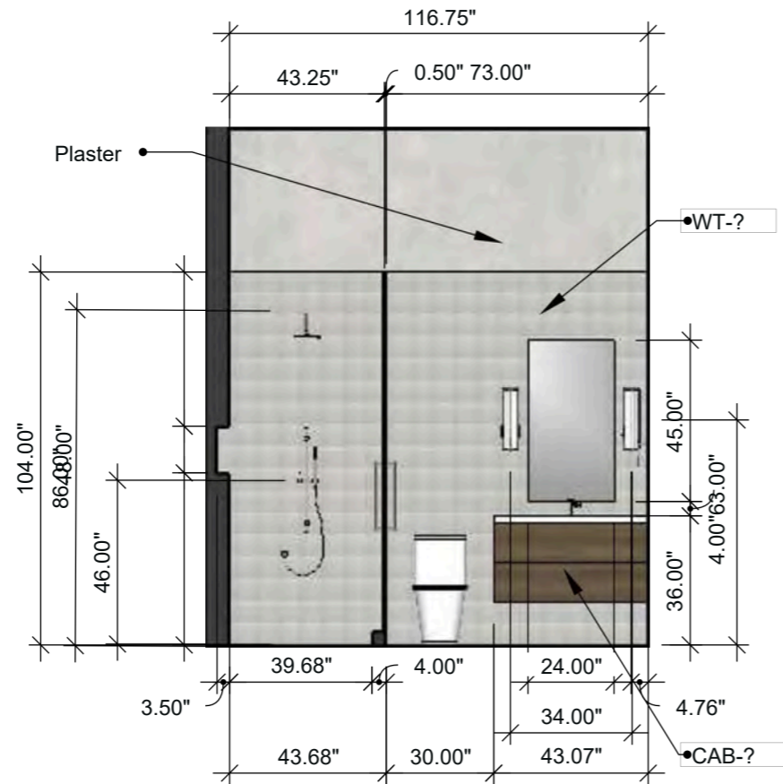
Outdoor Bath Elevation 1 SCALE: 1/4" = 1'-0" (1:48)
