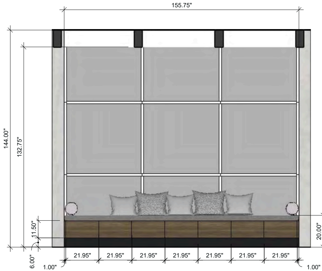
Dining Room Built-in Bench Elevation 1 SCALE: 3/8" = 1'-0" (1:32)
