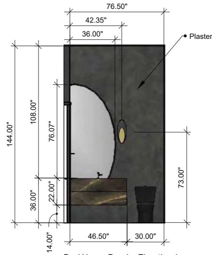
Pool House Powder Elevation 1 SCALE: 1/4" = 1'-0" (1:48)
