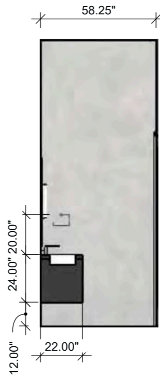
Outdoor Bath Elevation 2 SCALE: 1/4" = 1'-0" (1:48)
