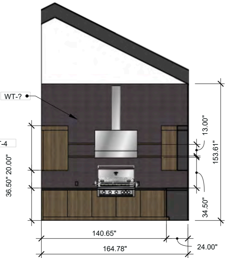
Outdoor Kitchen Elevation 1 SCALE: 3/16" = 1'-0" (1:64)
