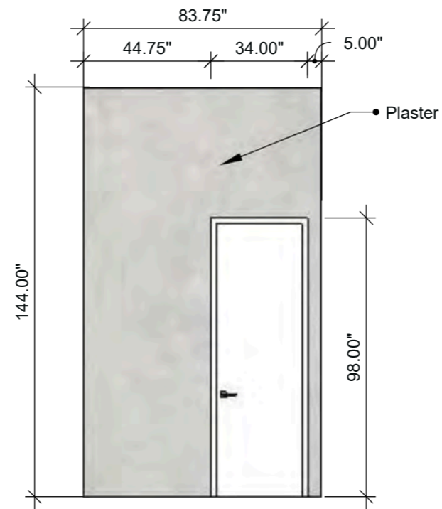
Powder Elevation 3 SCALE: 1/4" = 1'-0" (1:48)
