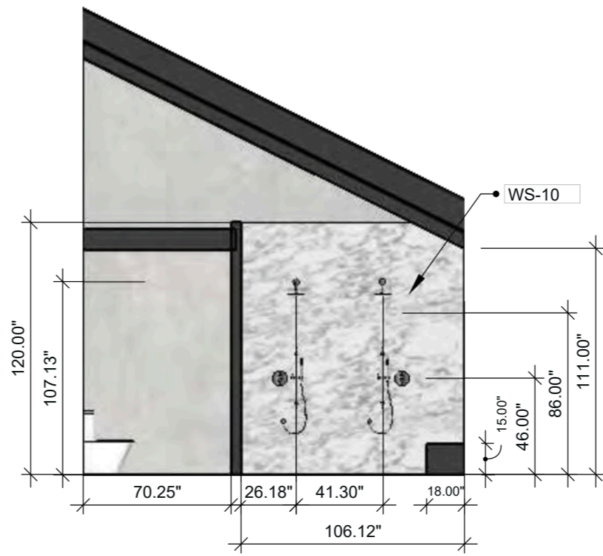
Primary Bath Elevation 2 SCALE: 3/16" = 1'-0" (1:64)
