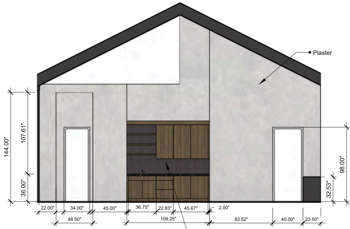
Pool House Kitchenette Elevation 1 SCALE: 3/16" = 1'-0" (1:64)
