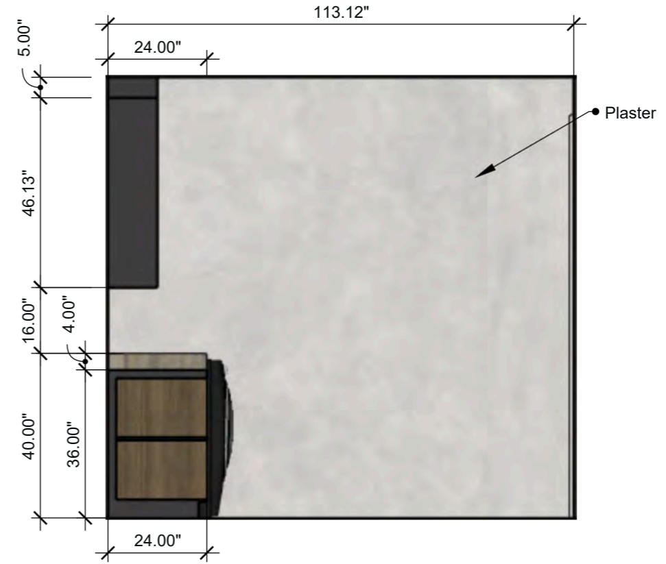
Laundry Elevation 2 SCALE: 3/8" = 1'-0" (1:32)
