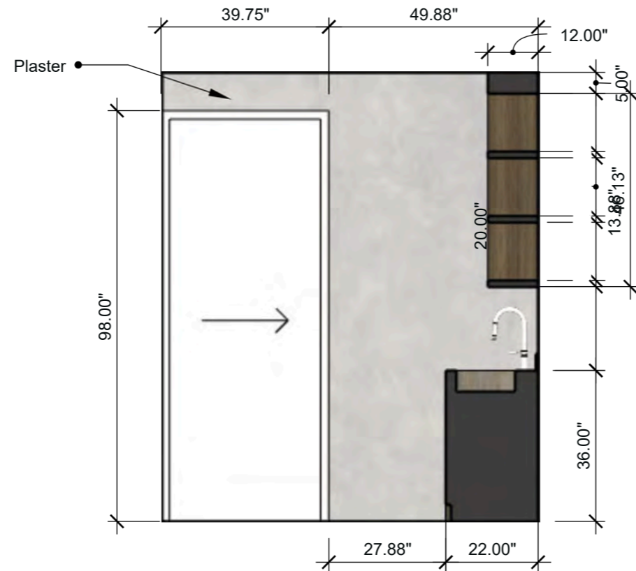
Laundry Elevation 3 SCALE: 3/8" = 1'-0" (1:32)
