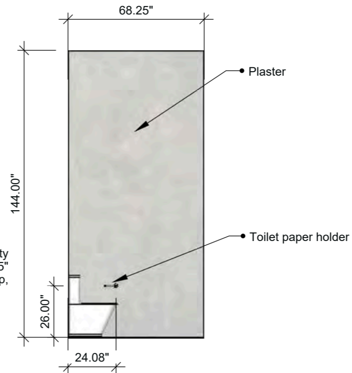
Powder Elevation 2 SCALE: 1/4" = 1'-0" (1:48)
