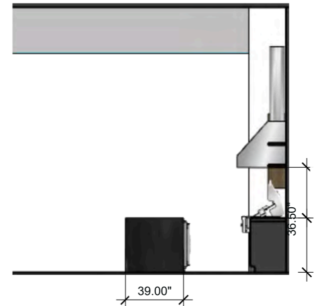
Outdoor Kitchen Elevation 4 SCALE: 3/16" = 1'-0" (1:64)
