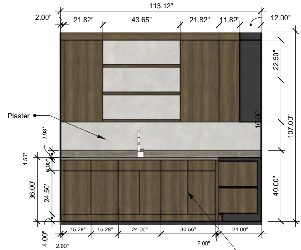
Laundry Elevation 4 SCALE: 3/8" = 1'-0" (1:32)
