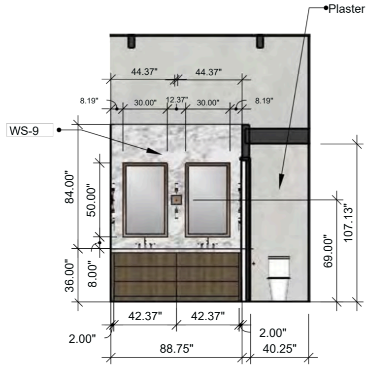
Primary Bath Elevation 1 SCALE: 3/16" = 1'-0" (1:64)
