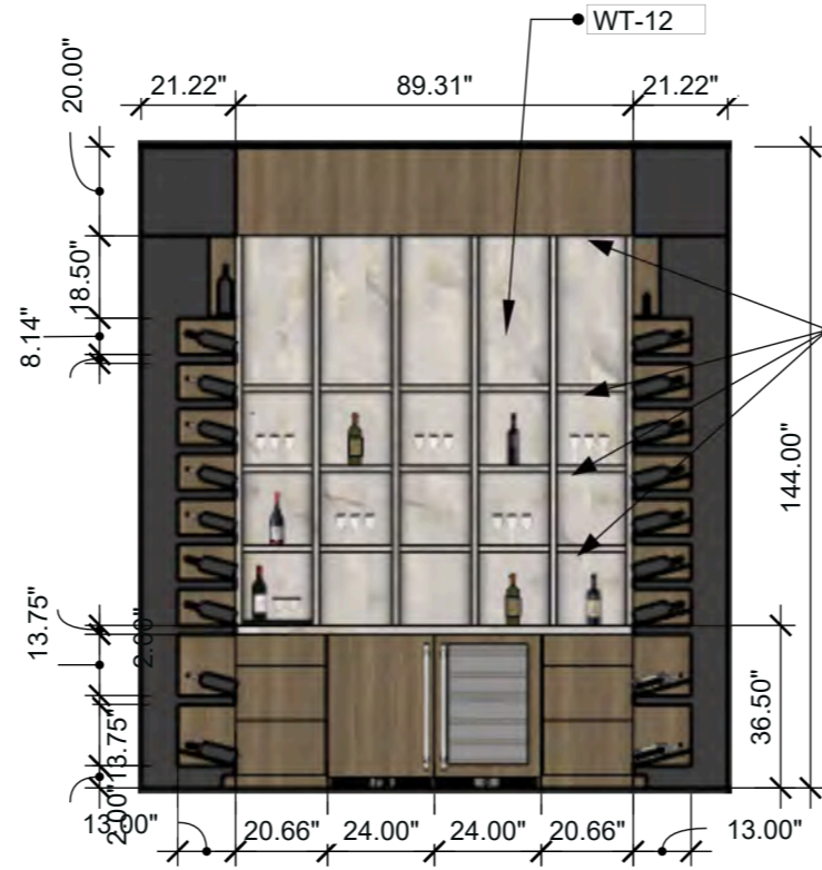
Wine Room Elevation 1 SCALE: 1/4" = 1'-0" (1:48)
