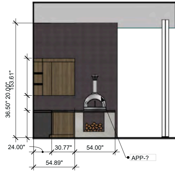
Outdoor Kitchen Elevation 2 SCALE: 3/16" = 1'-0" (1:64)
