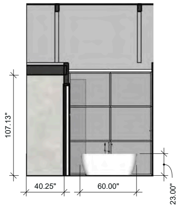
Primary Bath Elevation 3.1 SCALE: 3/16" = 1'-0" (1:64)
