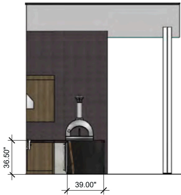
Outdoor Kitchen Elevation 2.1 SCALE: 3/16" = 1'-0" (1:64)
