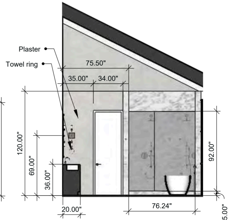
Primary Bath Elevation 2.1 SCALE: 3/16" = 1'-0" (1:64)
