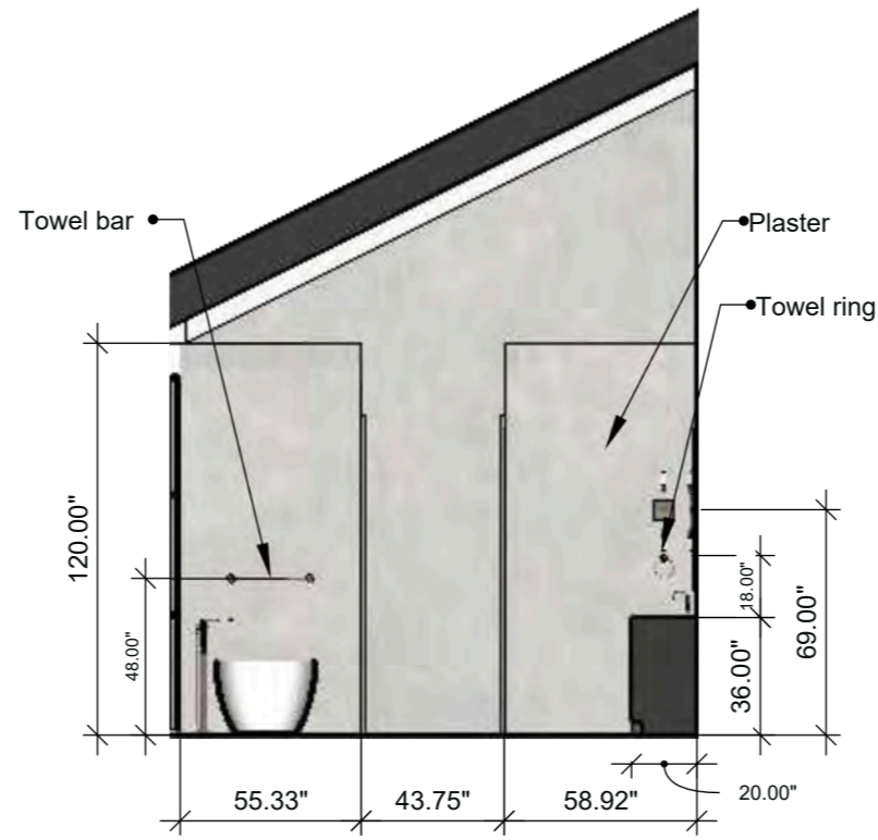
Primary Bath Elevation 4 SCALE: 3/16" = 1'-0" (1:64)
