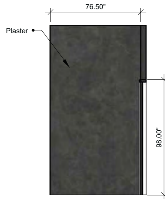
Pool House Powder Elevation 3 SCALE: 1/4" = 1'-0" (1:48)
