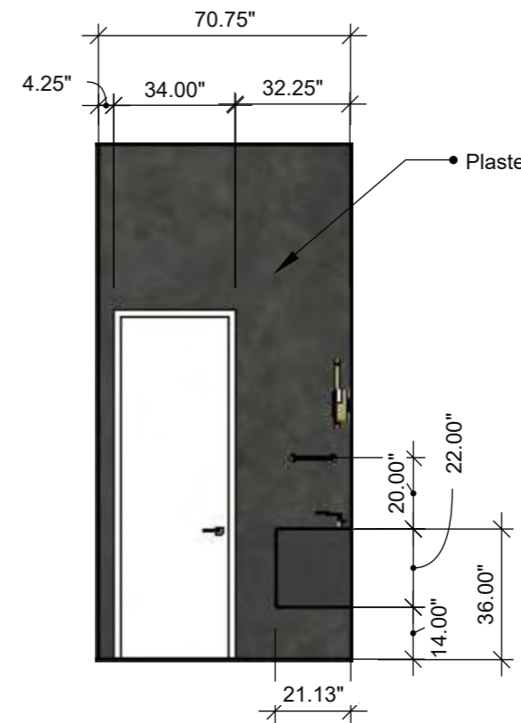
Pool House Powder Elevation 4 SCALE: 1/4" = 1'-0" (1:48)
