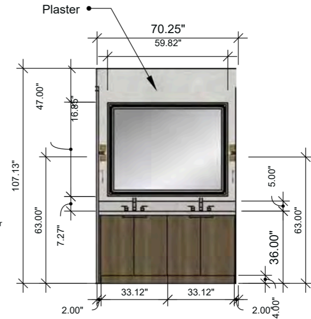
Shared Bath 1 & 2 Elevation 2.1 SCALE: 1/4" = 1'-0" (1:48)
