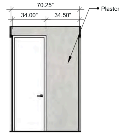
Shared Bath 1 & 2 Elevation 4 SCALE: 1/4" = 1'-0" (1:48)
