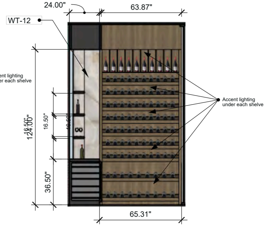
Wine Room Elevation 2 SCALE: 1/4" = 1'-0" (1:48)
