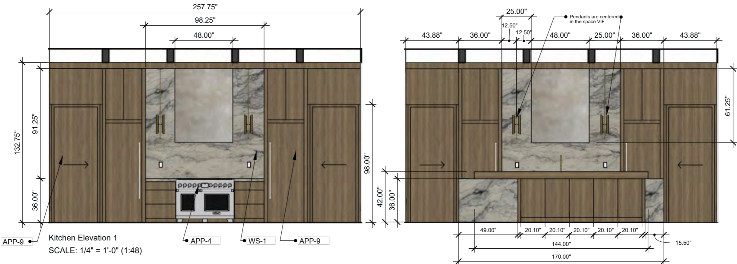
Kitchen Elevation 1.1 SCALE: 1/4" = 1'-0" (1:48)
