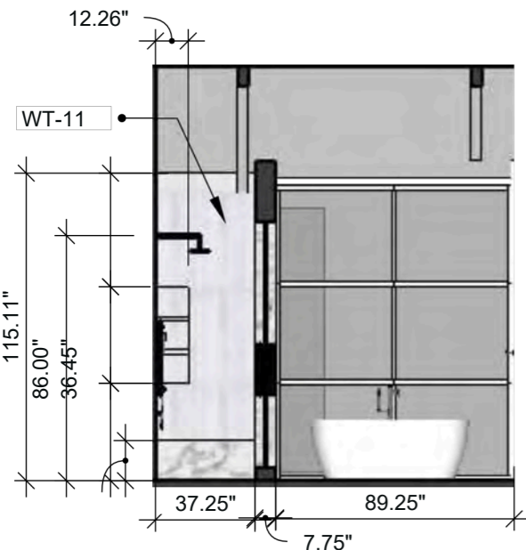
Primary Bath Elevation 3 SCALE: 3/16" = 1'-0" (1:64)
