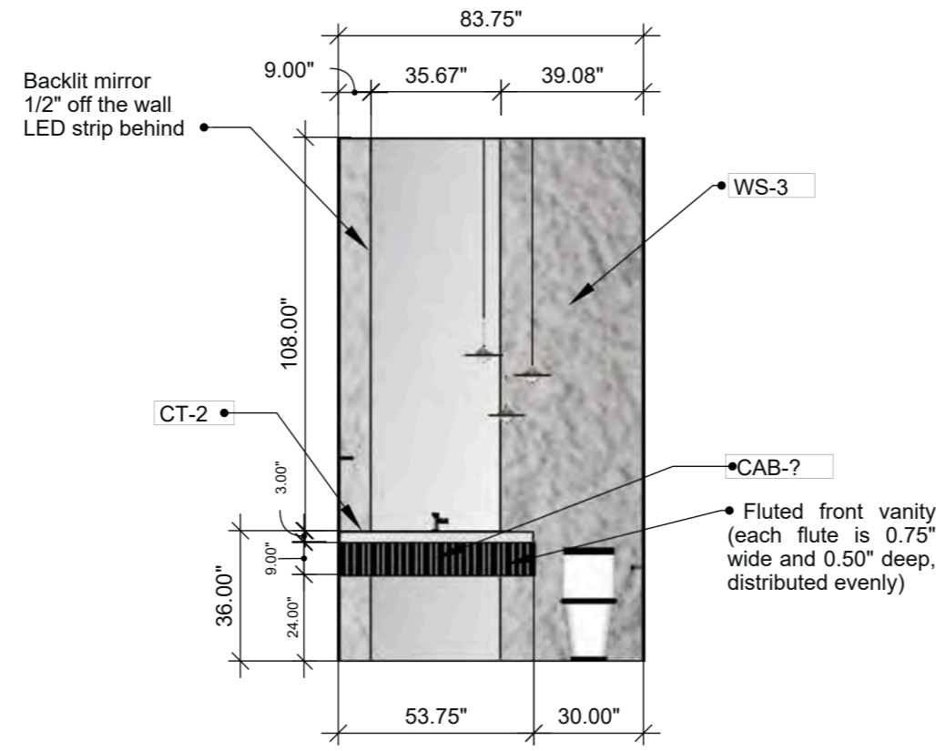
Powder Elevation 1 SCALE: 1/4" = 1'-0" (1:48)
