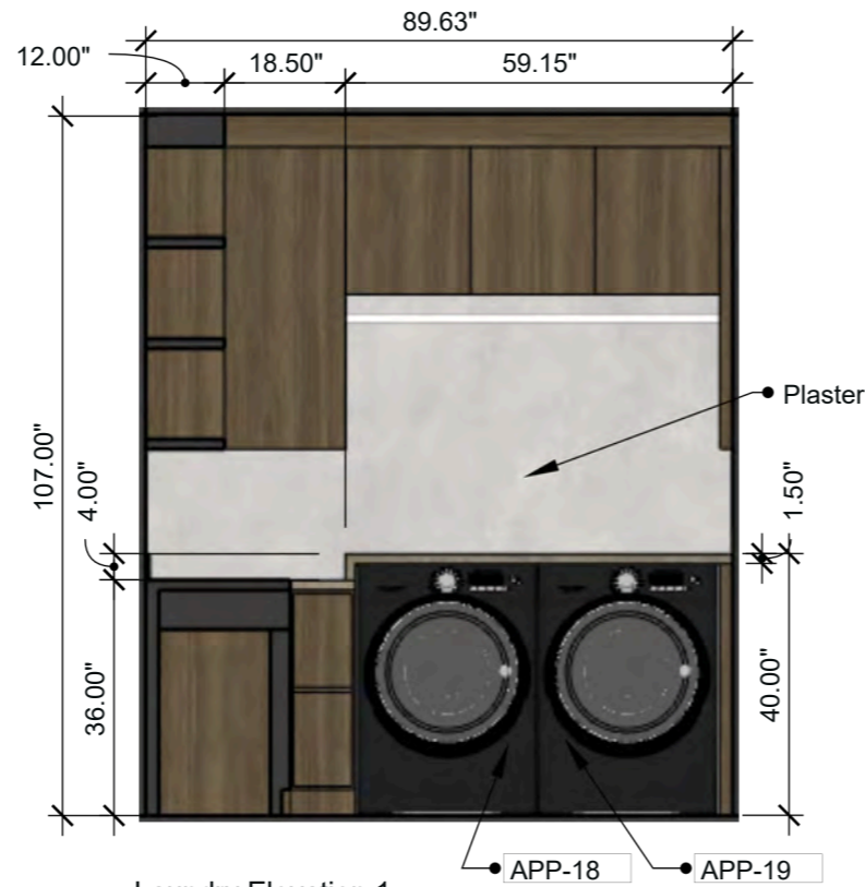
Laundry Elevation 1 SCALE: 3/8" = 1'-0" (1:32)
