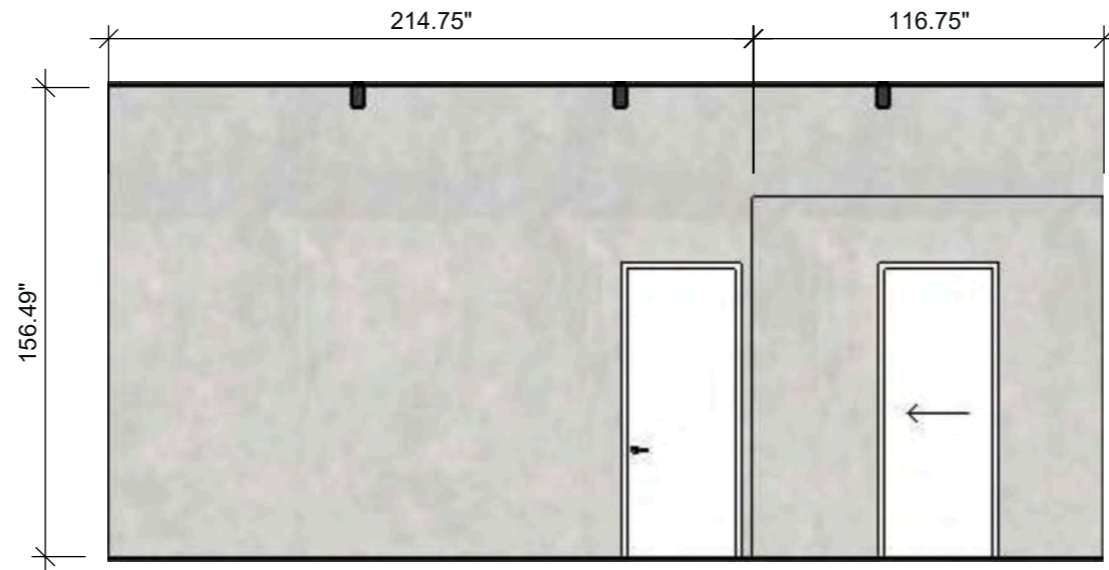
Primary Bedroom Elevation 3 SCALE: 3/16" = 1'-0" (1:64)
