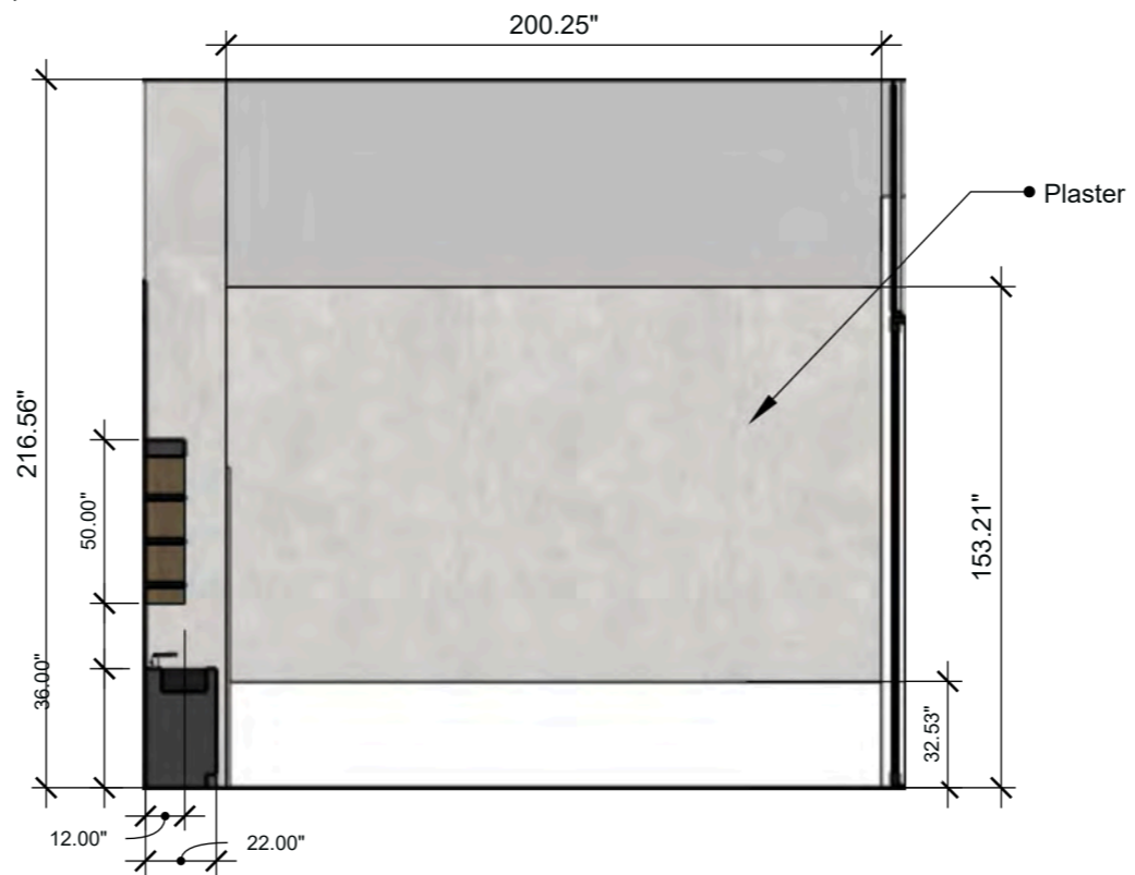
Pool House Kitchenette Elevation 3 SCALE: 3/16" = 1'-0" (1:64)
