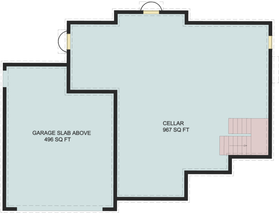
FOUNDATION PLAN
