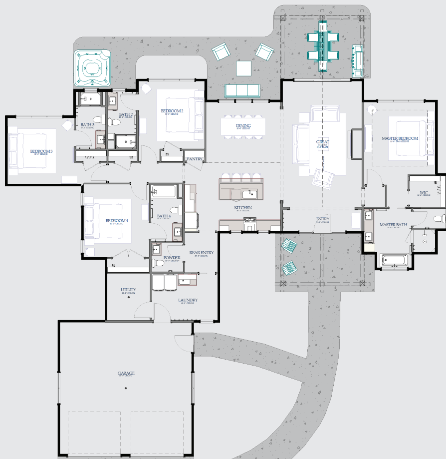
Main Level
