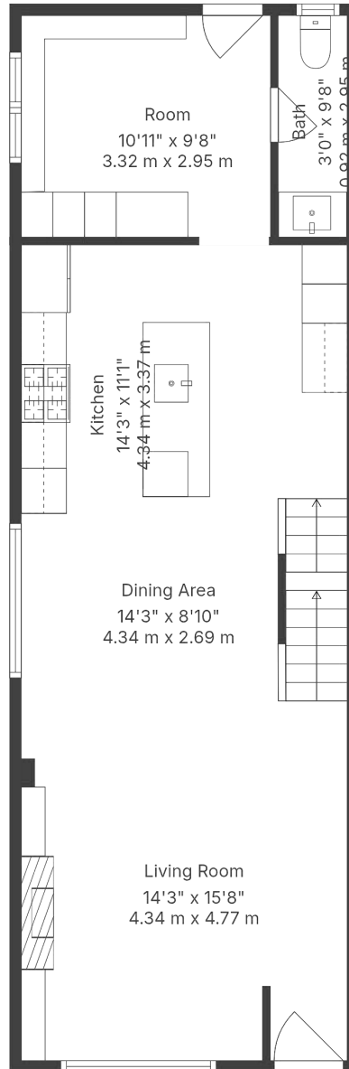
1st Floor
