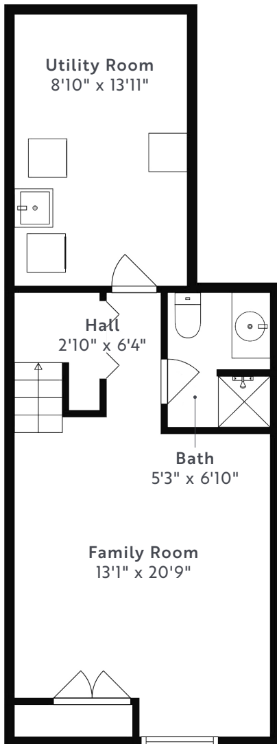
Basement
