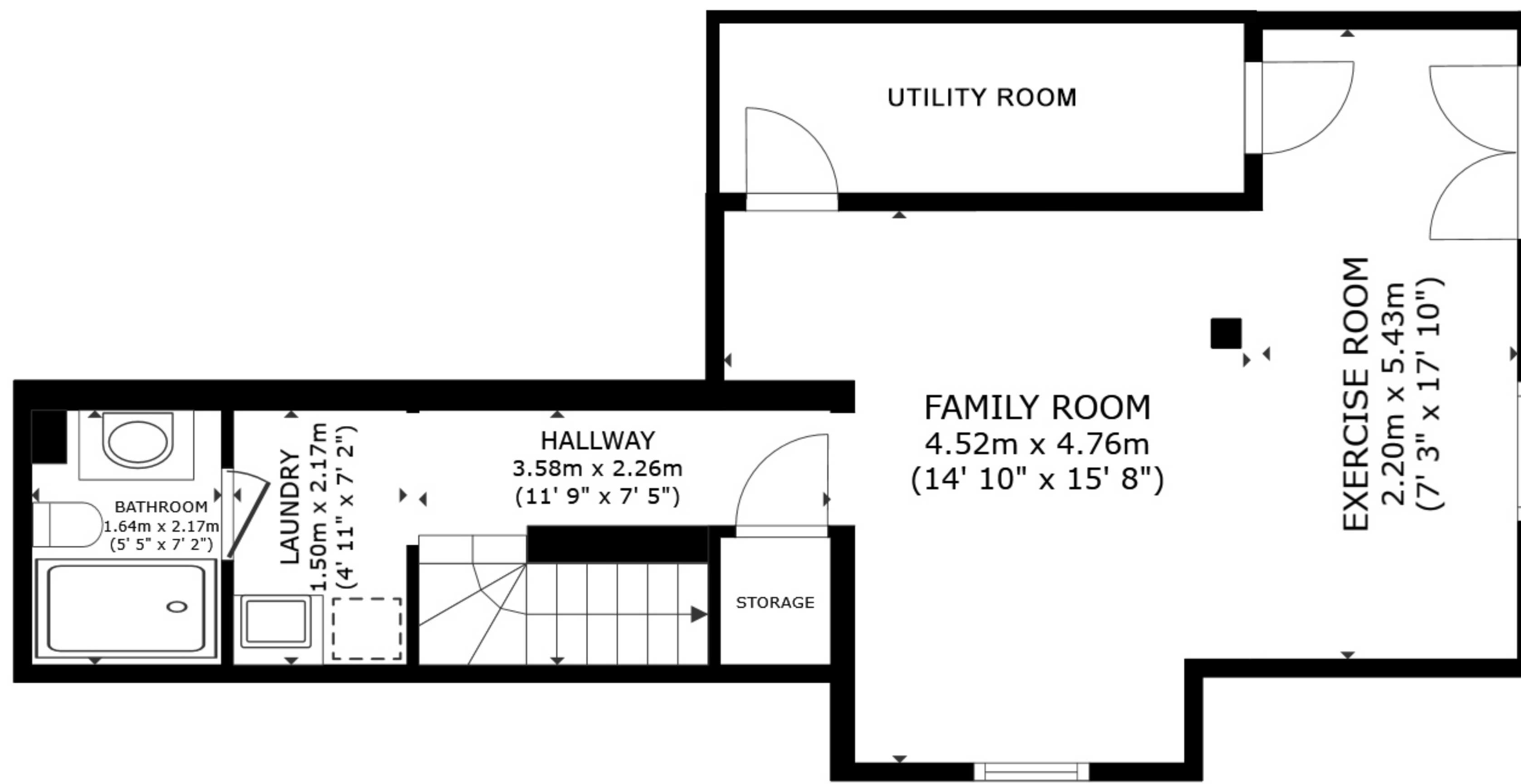
FLOOR 1
