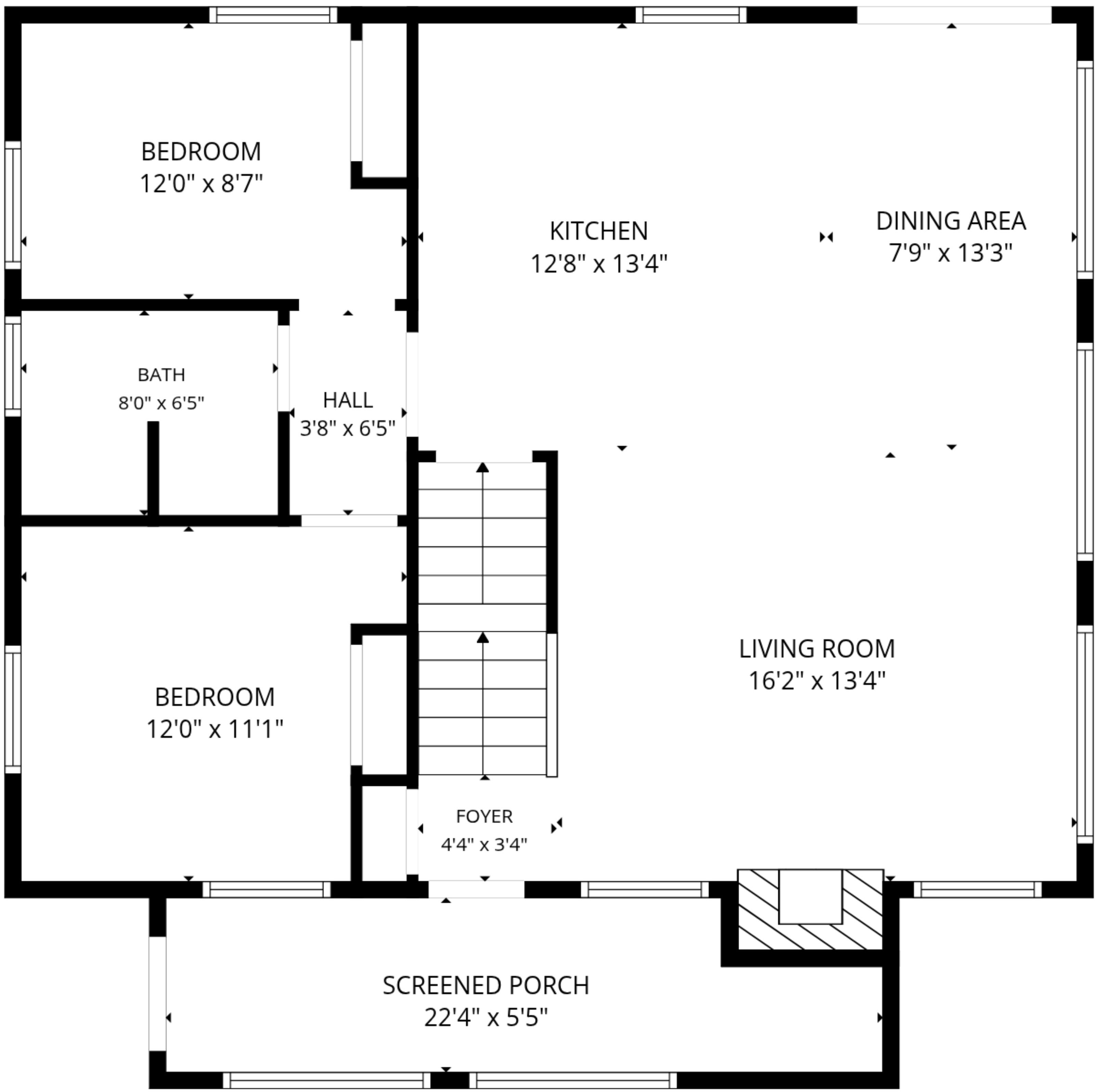
1st floor
