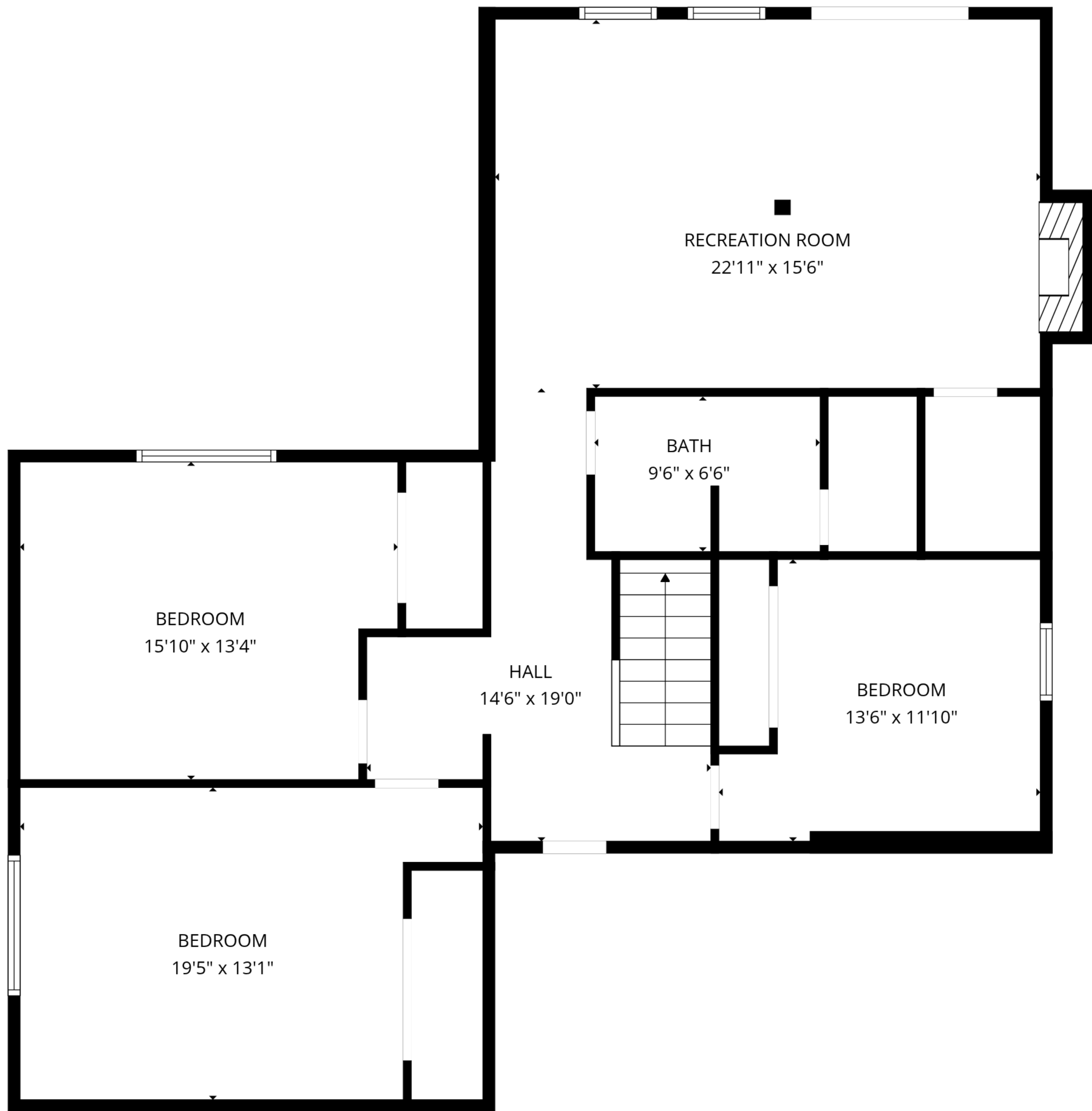
1st floor
