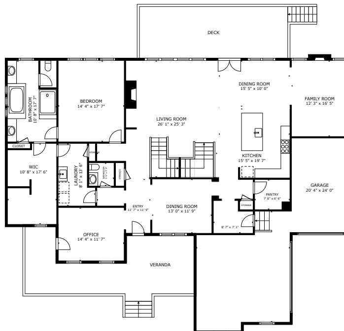
FLOOR 2
