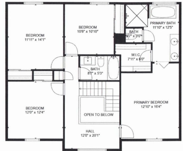
FLOOR 3
