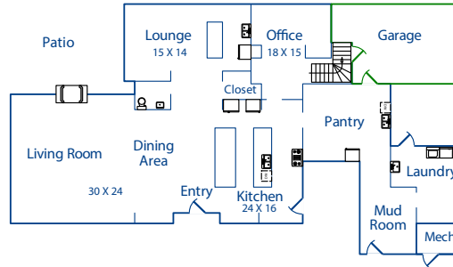
Upper Level
