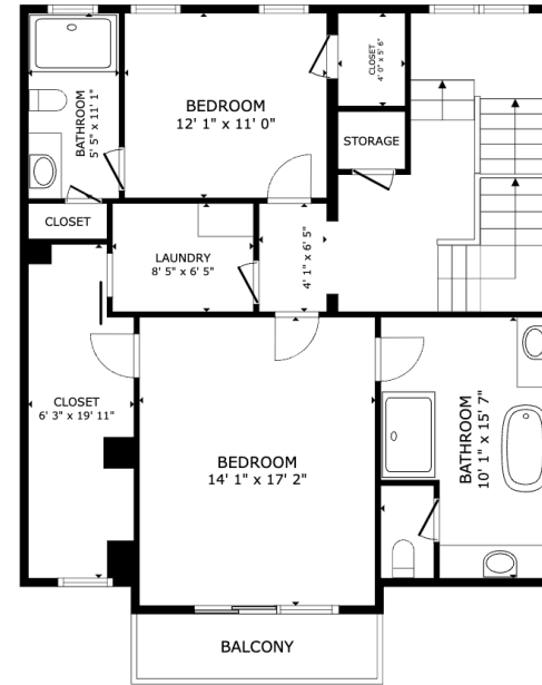
FLOOR 3
