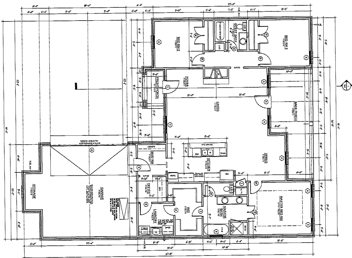
FLOOR PLAN
