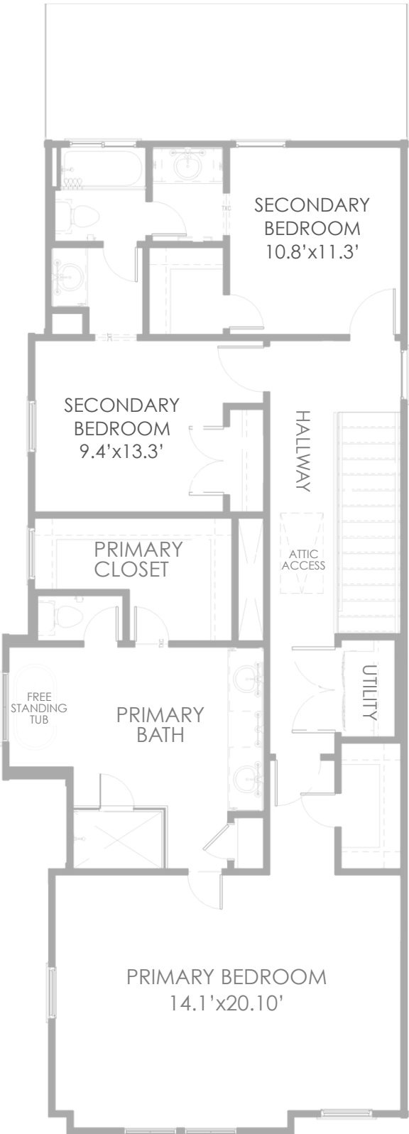
Second Floor
