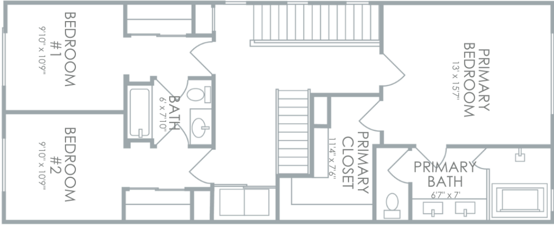
2ND FLOOR
