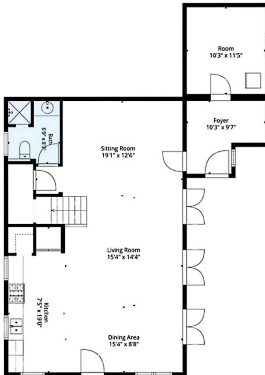
1st Floor
