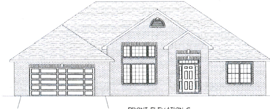
FRONT ELEVATION C
