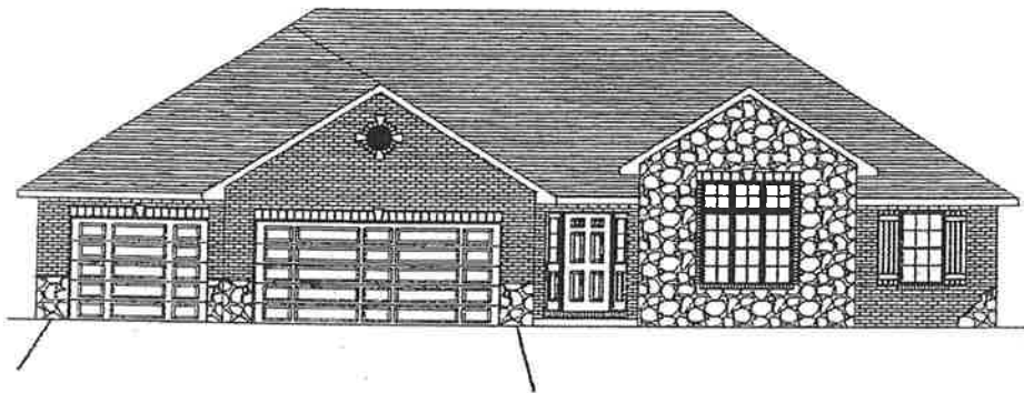
FRONT ELEVATION 'B'
