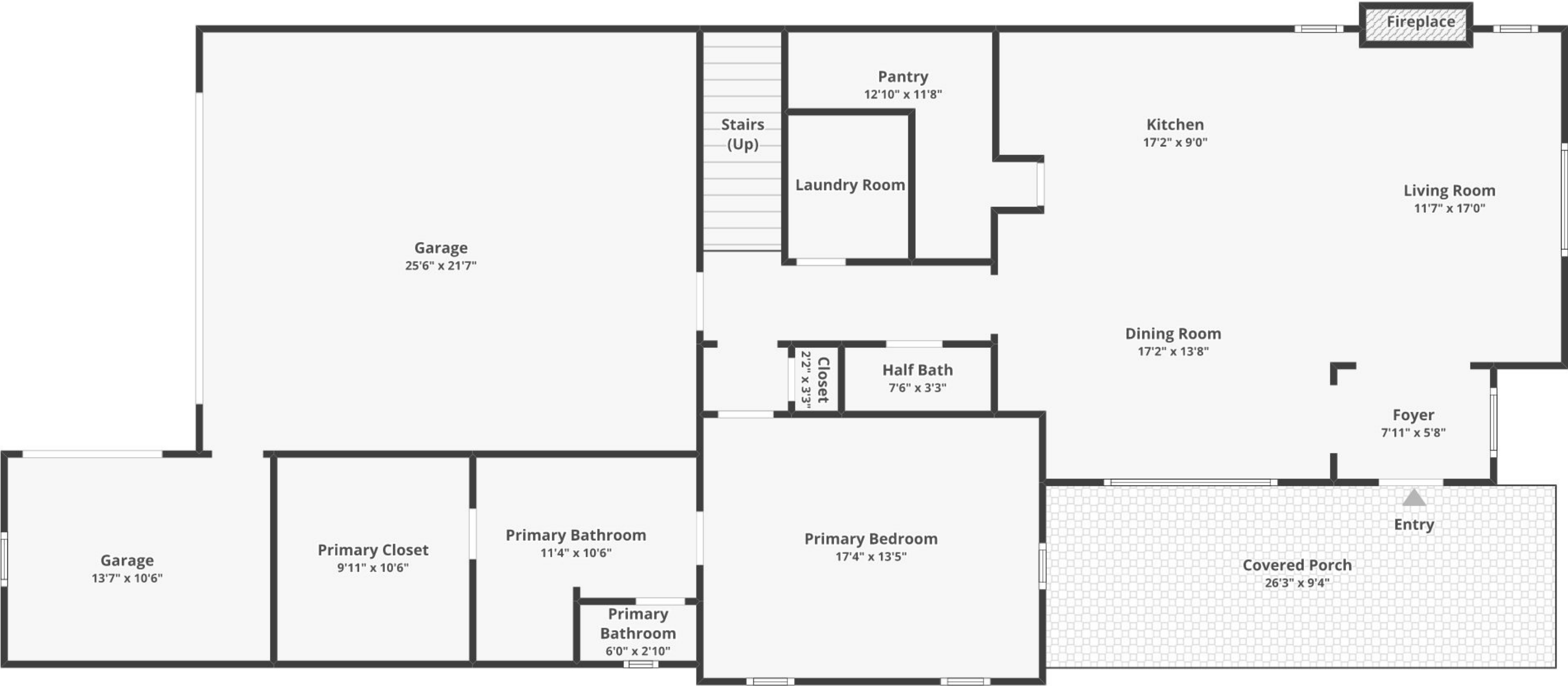
FLOOR 1
