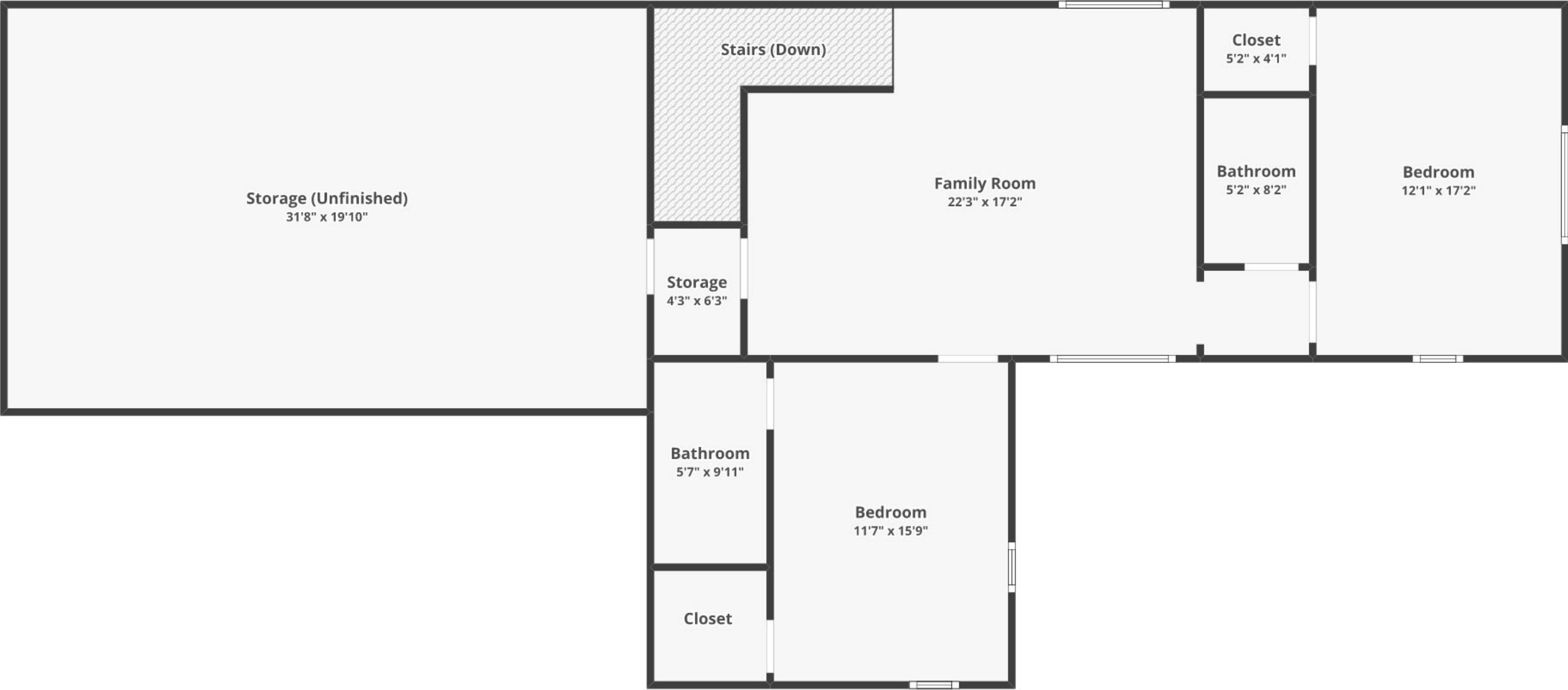
FLOOR 2
